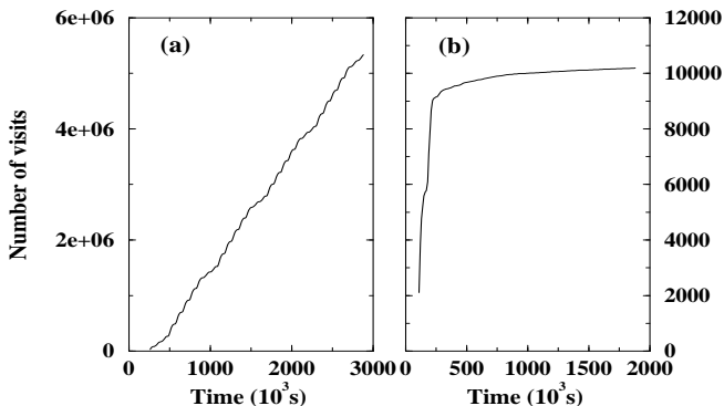
FIG. 1. The cumulative number of visits to a typical skeleton document (a) and a news document (b). The difference between the two visitation patterns allows us to distinguish between news documents and the stable documents belonging to the skeleton.
