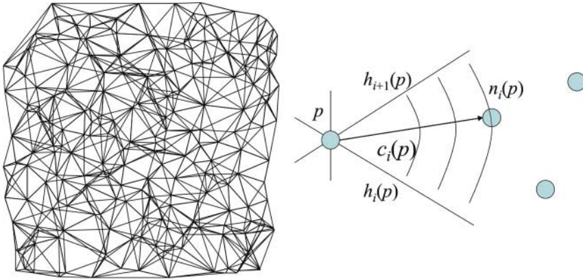
Fig. 2a. Yao graph for k = 6 with 256 nodes distributed uniformly at random within a square Fig. 2b. Sector c_i(p) with nearest neighbor n_i(p)
